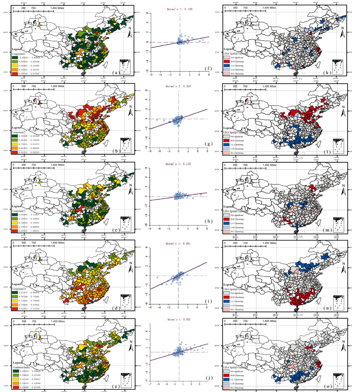
Fig. 6. Spatial distribution and spatial autocorrelation calculation results of urban carbon emission drivers ( p < 0.05 , from top to bottom, F_1 : economy-driven indicator, F_2 : environment-driven indicator, F_3 : industry-driven indicator, F_4 : resource-driven indicator and CI: composite index; from left to right, respectively, indicator distribution, Moran index, and LISA test results. The x-axis of the Moran index represents the observed values for each principal component and the y-axis represents the spatial lag of observed values.).
