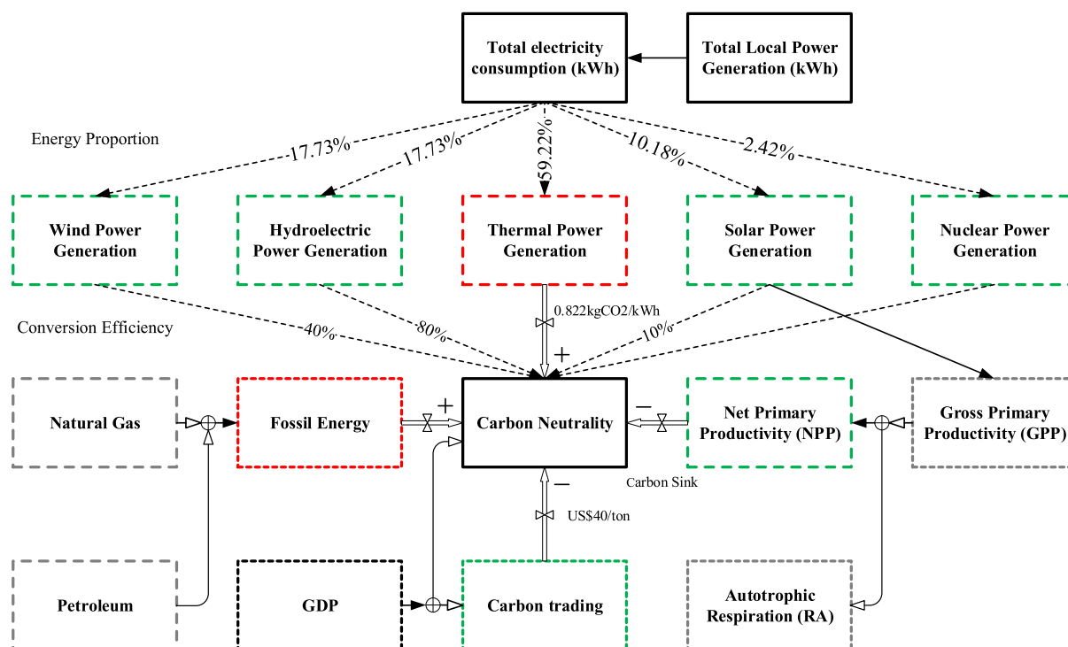
Fig. 1. Carbon footprints and energy calculation framework (Green boxes represent a disincentive to carbon emissions Red boxes represent a contribution to carbon emissions). (For interpretation of the references to color in this figure legend, the reader is referred to the web version of this article.)
