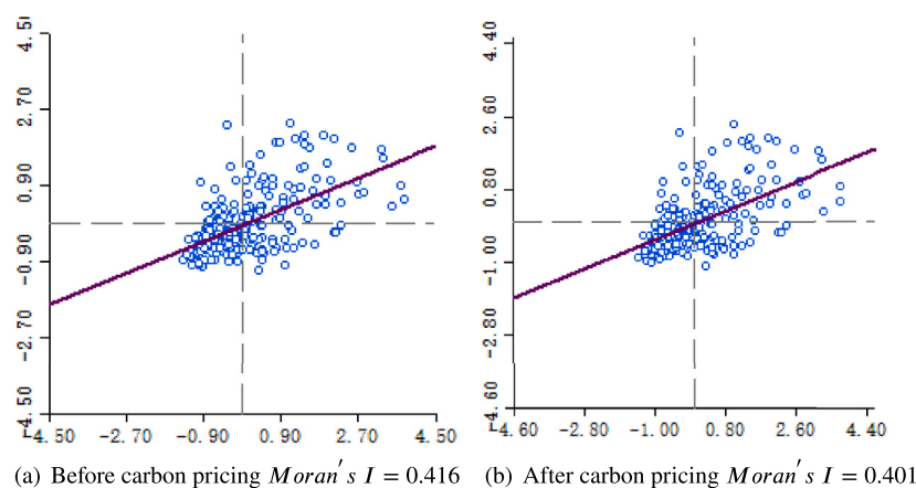
Fig. 3. Measuring the spatial auto-correlation of GDP per capita (The x-axis represents urban GDP per capita, the y-axis represents the spatial lag calculated based on Eq. (5) and Geoda 1.20 software.)
