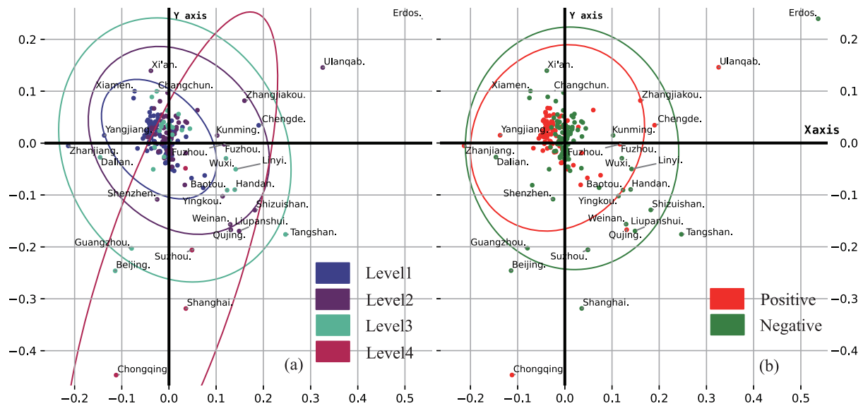
Fig. 4. T-SNE reduced dimensional presentation of cities with confidence ellipse distribution (a indicates the intensity of carbon emissions in different cities, and are categorized into 4 levels from low to high; b indicates whether the city benefits or loses from carbon pricing/carbon markets, i.e. positive vs. negative cities).
