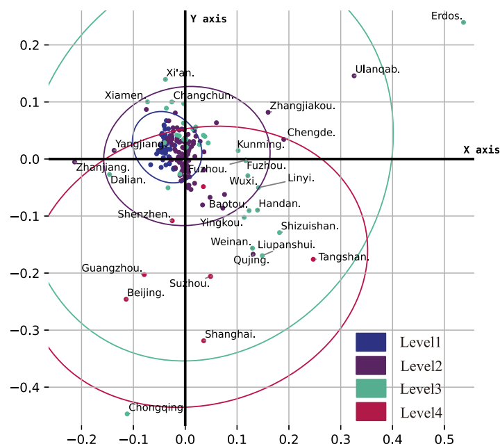
Fig. 7. Distribution of CI indicators for cities considering carbon sequestration and substitution capacity (using the natural breakpoint classification, the CI indicators are categorized into 4 levels from low to high).
