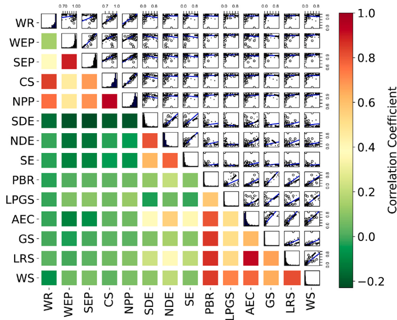
Fig. 5. Correlation of indicators and linear fitting results (Water Resource (WR), Wind energy potential (WEP), Solar energy potential (SEP), Carbon Sequestration (CS), Net Primary Productivity (NPP), Public Budget Revenue (PBR), Sulphur Dioxide Emission (SDE), Nitrogen Dioxide Emission (NDE), Industrial Soot Emission (SE), Liquefied Petroleum Gas Supply (LPGS), Annual Electricity Consumption (AEC), Gas Supply (GS), Luminous remote sensing image brightness values (LRS), Water Supply (WS)).
