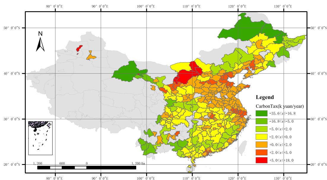
Fig. 2. Spatial distribution of the carbon tax to be paid by each city in China (the greenish color represents carbon surplus, the reddish color represents carbon deficit, and the different colors indicate the amount of carbon tax the city needs to pay per capita). (For interpretation of the references to color in this figure legend, the reader is referred to the web version of this article.)
