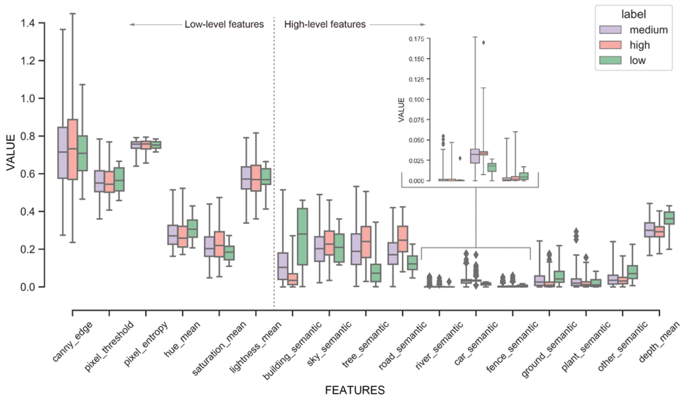
Fig. 6. Differences in visual characteristics of campus spaces at different restoration levels.
