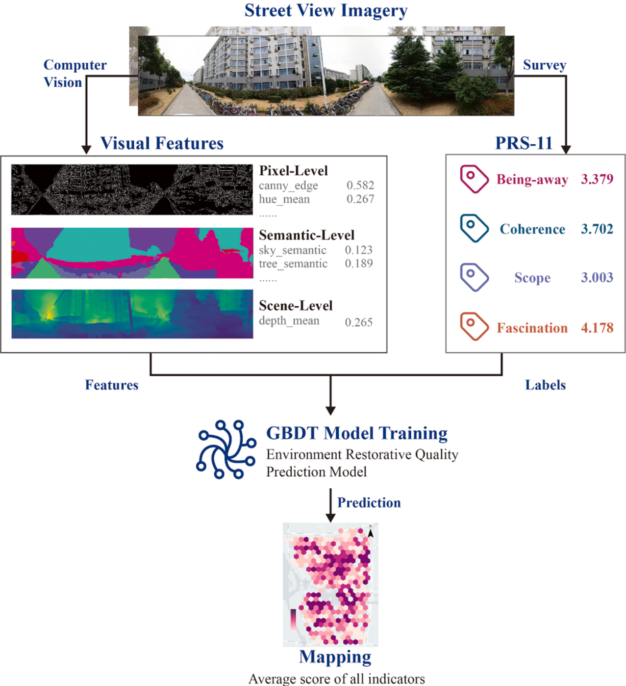
Fig. 1. Overview of our workflow to assess walking space on university campus restorative quality comprehensively from street view imagery.
