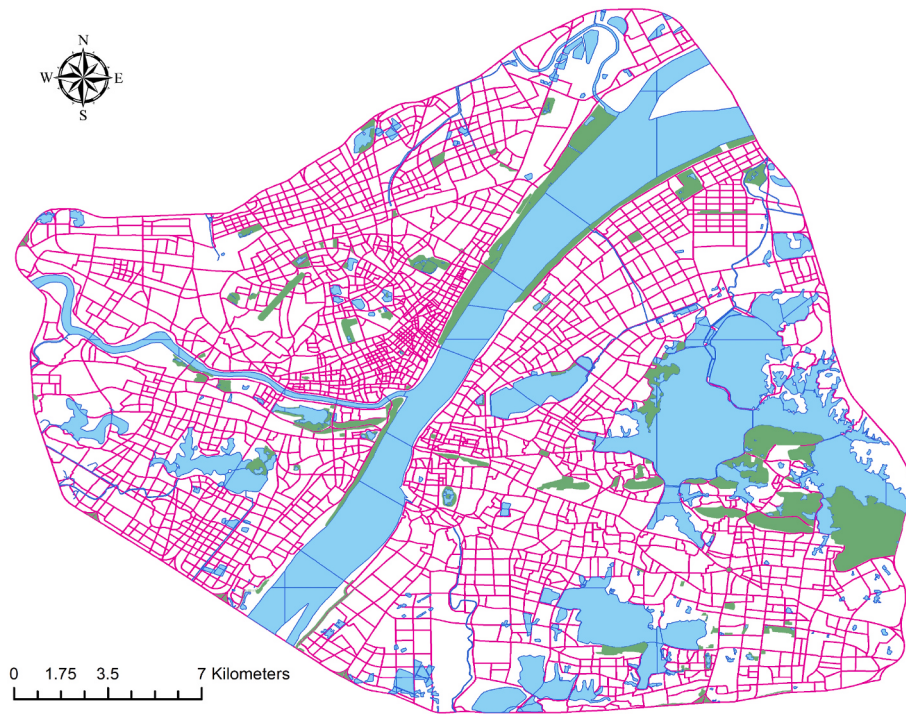
Fig. 1. Structure of Wuhan City's road network.
