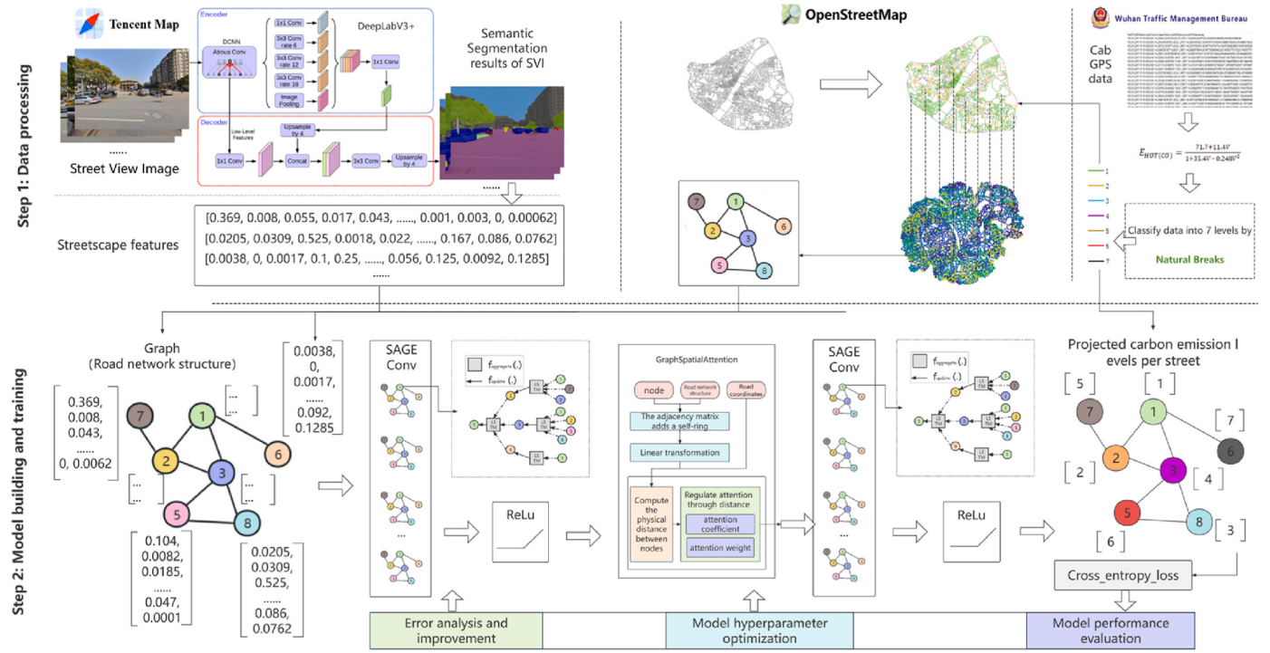
Fig. 6. Method of predicting CO emission levels. Step 1: Data processing. Step 2: Building and training the SAGE-GSAN model.
