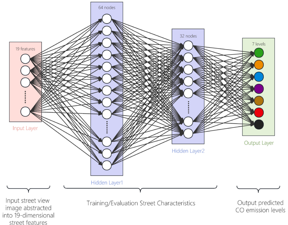
Fig. 8. MLP predicts street-level CO emissions.
