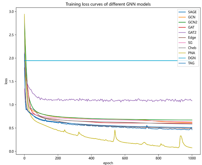
Fig. 10. Training loss curves for different models.
