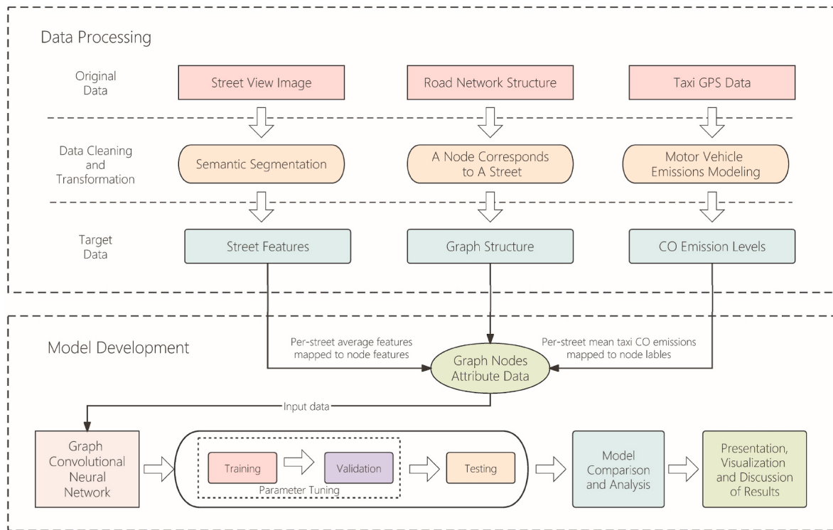
Fig. 4. Research framework diagram.
