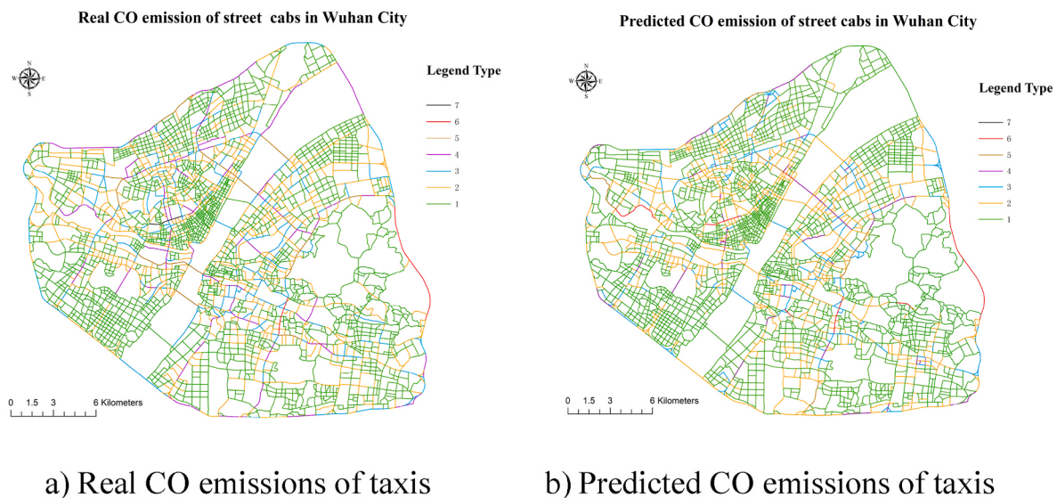
Fig. 7. Predictions of the SAGE-GSAN model regarding the street-level CO emissions of taxis. In the legend, Types 1–7 represent low to high levels of CO emissions. a) Real CO emissions of taxis b) Predicted CO emissions of taxis.
