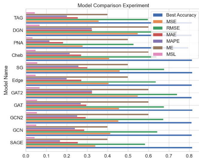
Fig. 9. Bar chart comparing the models' metrics.
