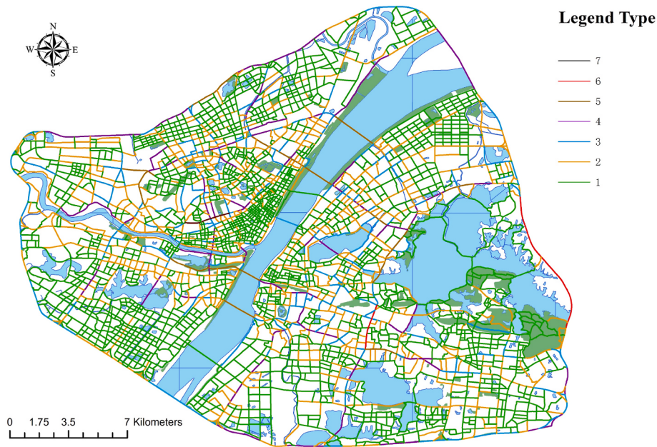
Fig. 3. CO emission levels of the roads classified by the natural breaks method.
